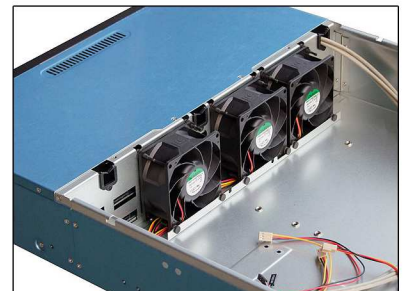
Three 80mm x 38mm Sunon 2ball bearing fans
