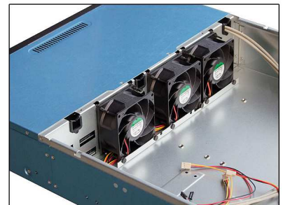
Three 80mm x 38mm Sunon 2ball bearing fans
