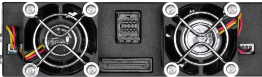
One SFF-8643 data transfer port
